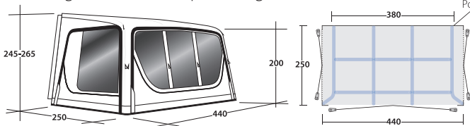
RIPPLE MOTOR 440SA M
