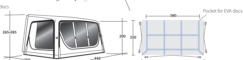
RIPPLE MOTOR 440SA L
