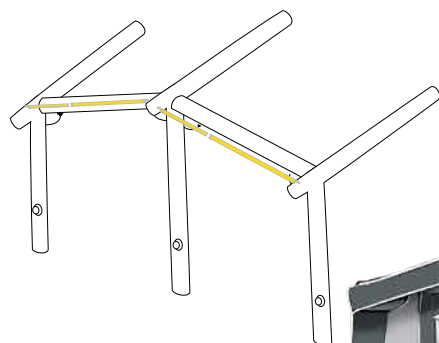
Horizon Air main frame system (additional roof support and storm tubes are supplied as standard on sizes 10-22)
