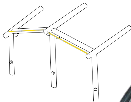
Daytona Air main frame system (additional roof support and storm tubes are supplied as standard on sizes 10-19)
